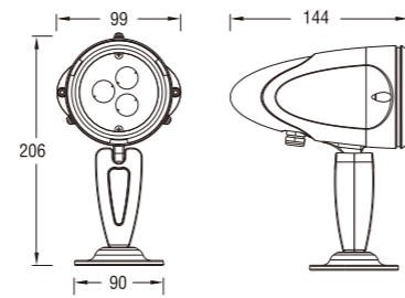
Product Dimension
