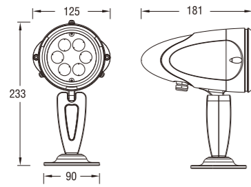
Product Dimension
